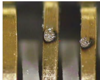
Spark Gap erosion shown located away from the critical contact area. Arcing is inevitable, but in a fully mated connection, the plug makes contact with the jack in the critical contact area, away from any spark gap erosion.
